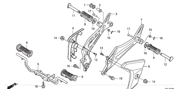
F-19 STEP
