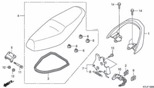
F-14 SEAT
