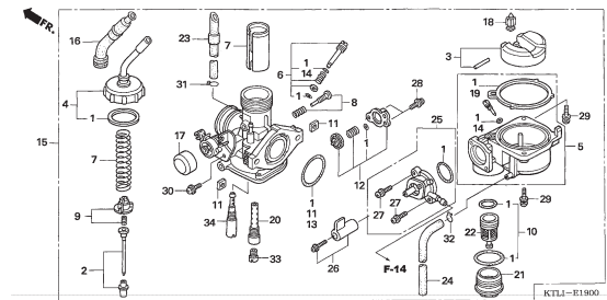
E-19 CARBURETOR
