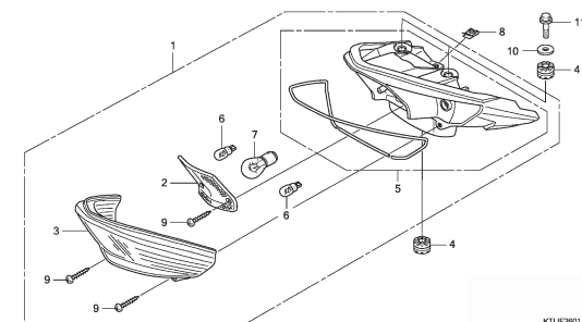
F-25 REAR COMBINATION LIGHT
