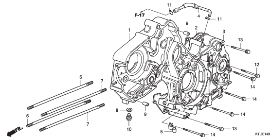
E-14 CRANKCASE
