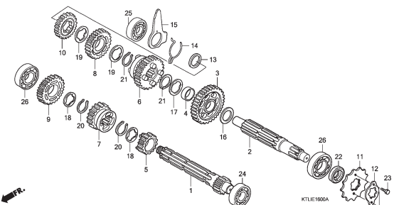
E-16 TRANSMISSION
