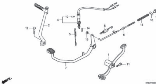
F-18 PEDAL/KICK STARTER ARM
