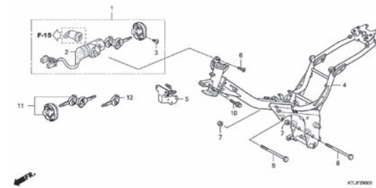
F-28 FRAME BODY
