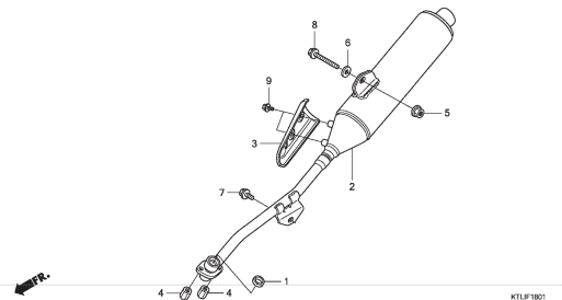
F-17 EXHAUST MUFFLER
