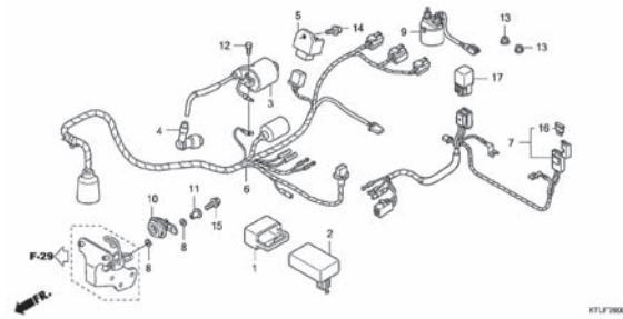
F-27 WIRE HARNESS
