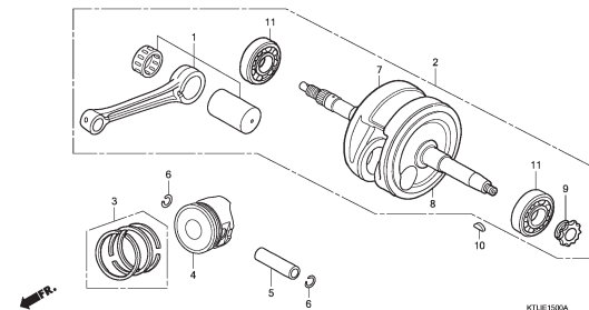
E-15 CRANKSHAFT/PISTON
