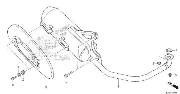
F-30 EXHAUST MUFFLER
