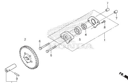
E-11 OIL PUMP
