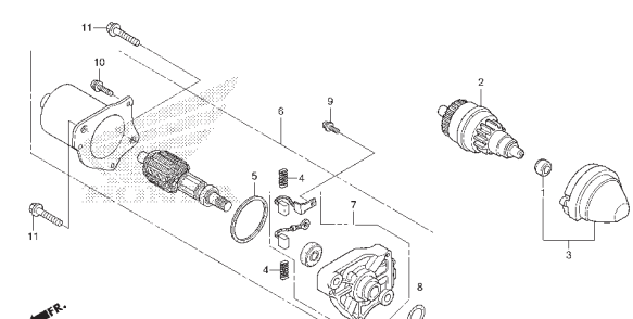
E-12 STARTING MOTOR
