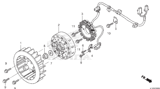
E-8 GENERATOR
