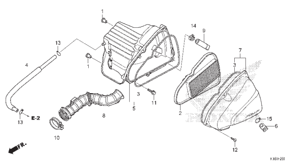
F-28 AIR CLEANER
