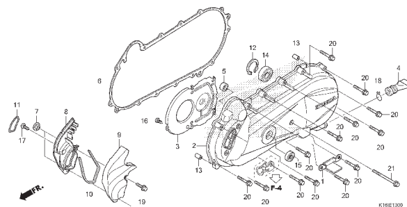
E-17-10 TRANSMISSION
