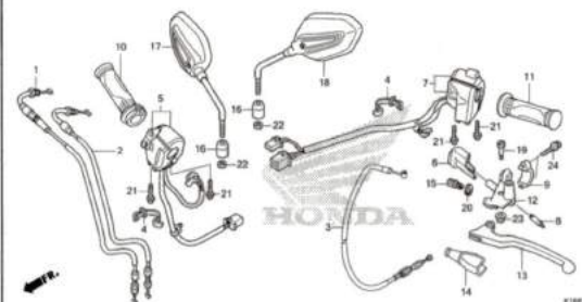
F-4 HANDLE LEVER/SWITCH/ CABLE/MIRROR
