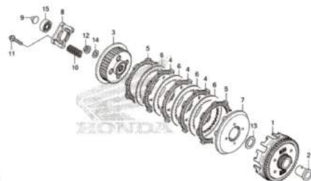
E-8 CLUTCH
