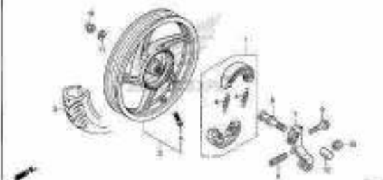
F-22-31 REAR WHEEL (ACI110CBG/H/J,CBTG/H/J)
