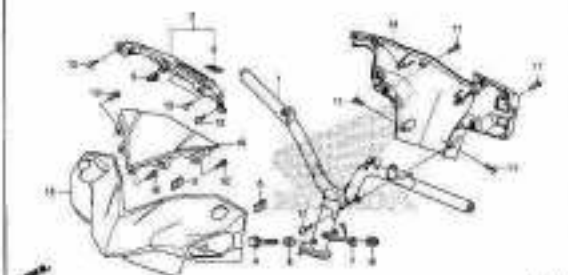
F-9-1 HANDLE PIPE/HANDLE COVER (ACI110CBG/H/J,CBTG/H/J)
