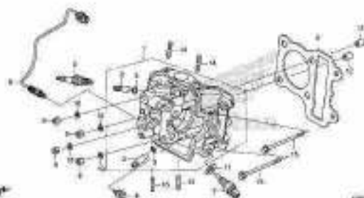
E-3 CYLINDER HEAD(ACI110CBE)
