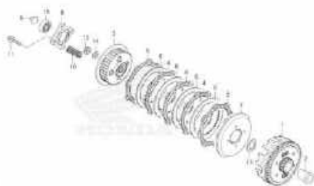
E-8 CLUTCH
