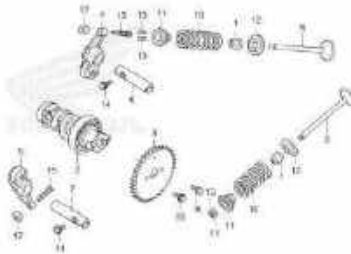
E-4 CAMSHAFT/VALVE
