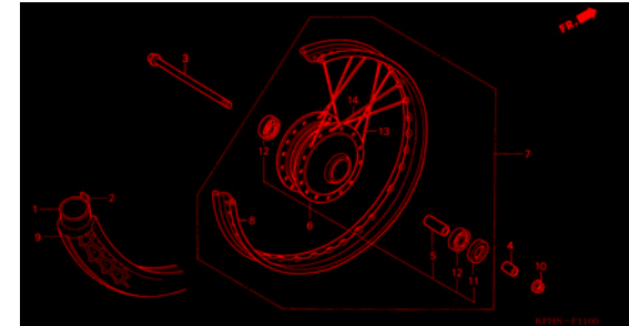
F-11 FRONT WHEEL (Type Drum Brake)
