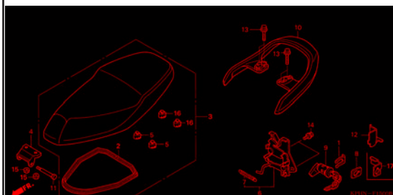
F-17 SEAT
