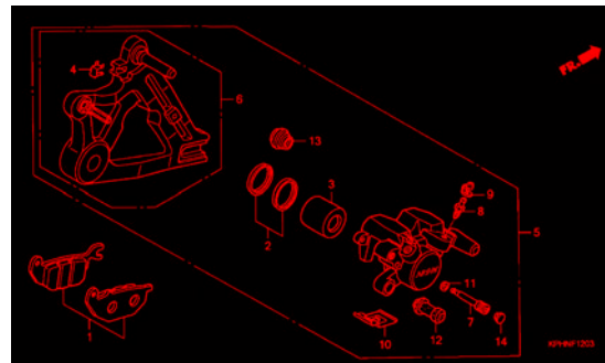
F-14 REAR BRAKE CALIPER
