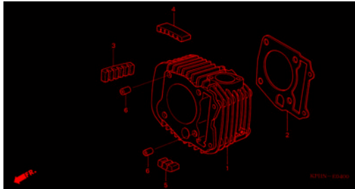
E-4 CYLINDER
