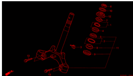
F-6 STEERING STEM
