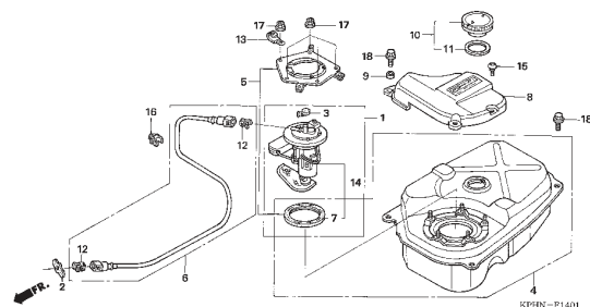
F-16-1 FUEL TANK Type PGM-FI
