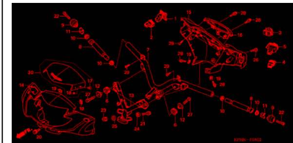
F-5 HANDLE PIPE/ HANDLE COVER /SWITCH
