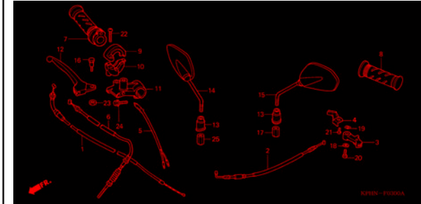
F-3 HANDLE LEVER / CABLE / MIRROR (Drum)
