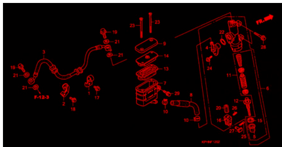
F-13 REAR BRAKE MASTER CYLINDER
