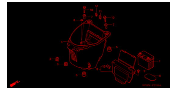
F-29 BATTERY / LUGGAGE BOX
