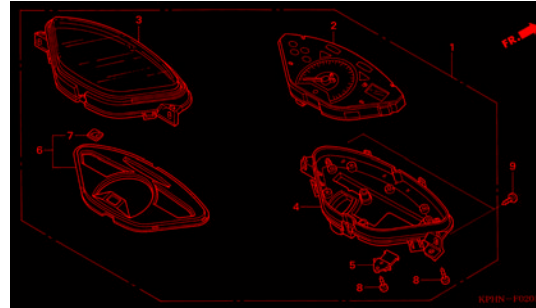
F-2 SPEEDOMETER
