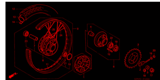
F-15 REAR WHEEL
