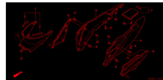
F-18 BODY COVER
