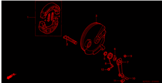
F-9 FRONT BRAKE PANEL
