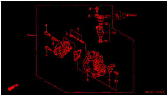
E-19 THROTTLE BODY type PGM - FI
