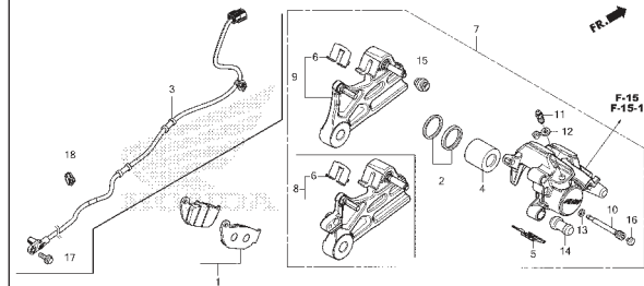
F-17 REAR BRAKE CALIPER
