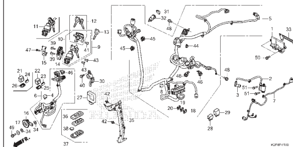
F-41 WIRE HARNESS(ACF110CBT-IN,3IN)
