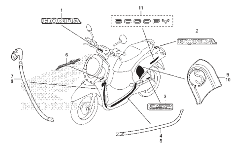
F-48-1 MARK/STRIPE(2)
