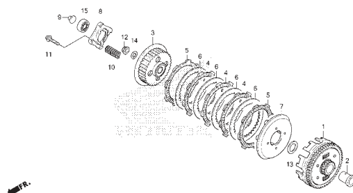
E-8 CLUTCH
