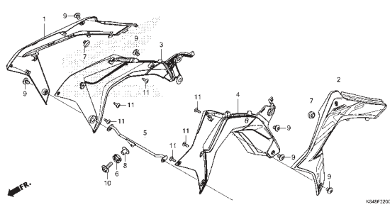
F-22 SHROUD
