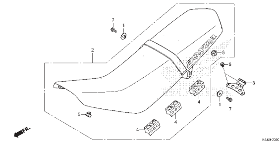
F-23 SEAT
