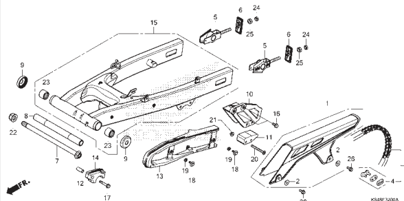
F-32 SWINGARM
