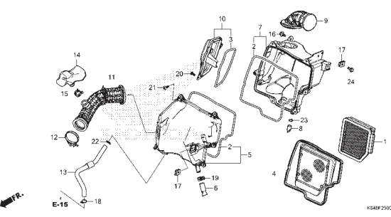
F-25 AIR CLEANER
