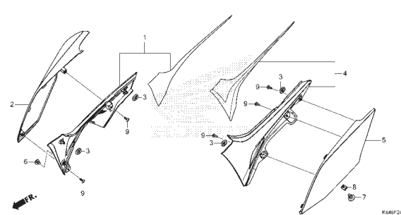
F-24 SIDE COVER
