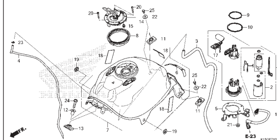
F-21-1 FUEL TANK(CB150RM)
