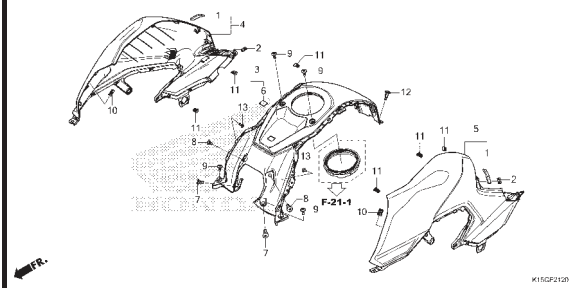
F-21-20 FUEL TANK COVER
