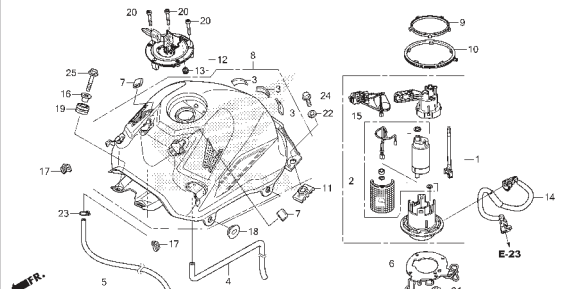
F-21 FUEL TANK (CB150RG/H/J/K/L)
