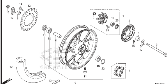
F-19-41 REAR WHEEL(CB150RM)
