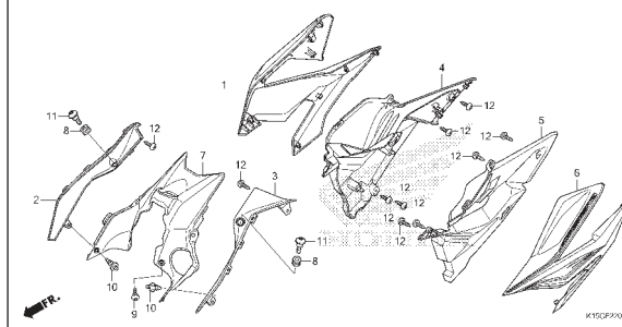
F-22-1 SHROUD(CB150RK/L)
