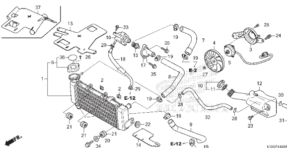
F-41 RADIATOR
