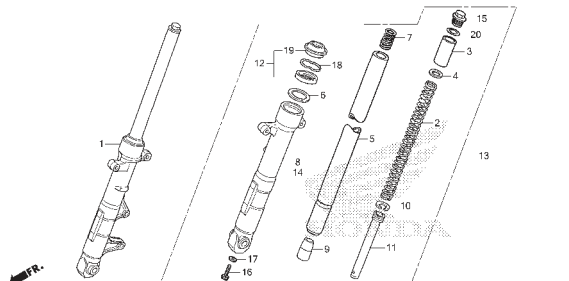
F-11 FRONT FORK(CB150RG/H/J/K/L)
