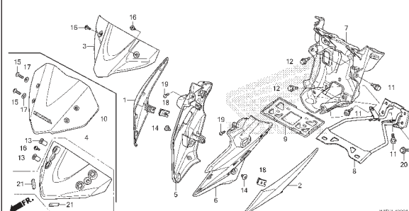
F-43 FRONT COWL(CB150RG/H/J/K/L)
