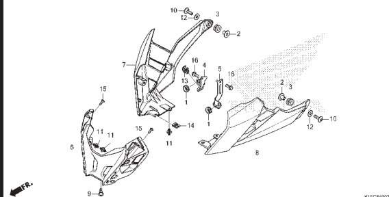
F-45-2 UNDER COWL(3)
