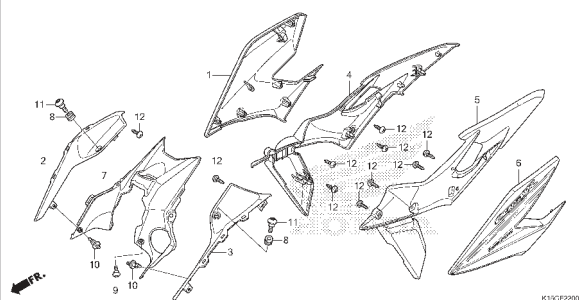
F-22 SHROUD(CB150RG/H/J)
