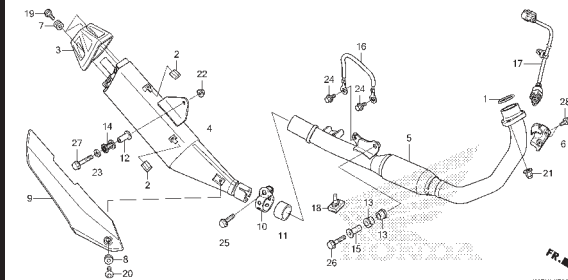
F-27 EXHAUST MUFFLER
