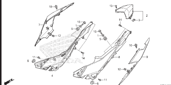
F-24-1 REAR COWL(CB150RK/L)
