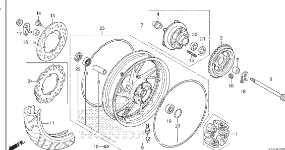
F-19-40 REAR WHEEL (CB150RG/H/J/K/L)
