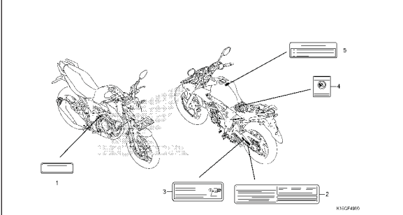
F-49 CAUTION LABEL (CB150RG/H/J/K/L)
