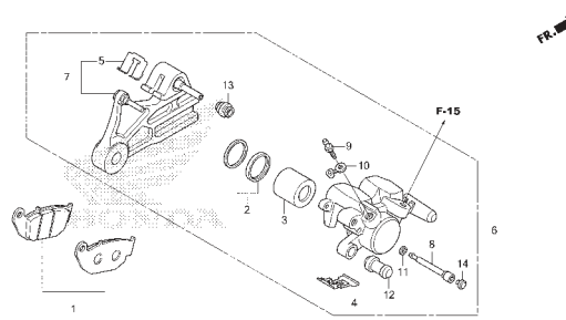
F-17 REAR BRAKE CALIPER
