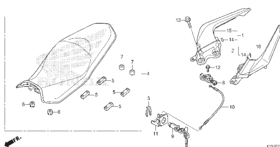
F-23 SEAT
