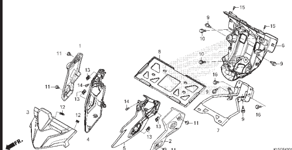
F-43-1 FRONT COWL(CB150RM)
