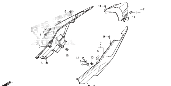
F-24-2 REAR COWL(CB150RM)
