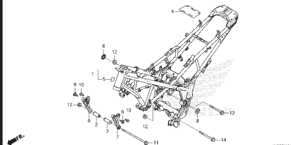
F-39-1 FRAME BODY(CB150RM)
