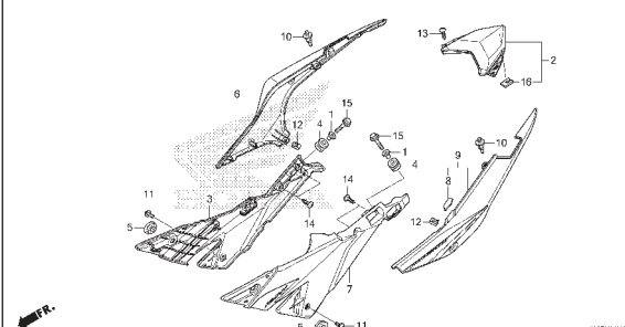
F-24 REAR COWL(CB150RG/H/J)
