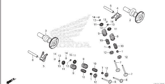
E-3 CAMSHAFT/VALVE
