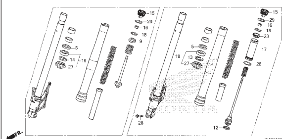
F-11-1 FRONT FORK(CB150RM)
