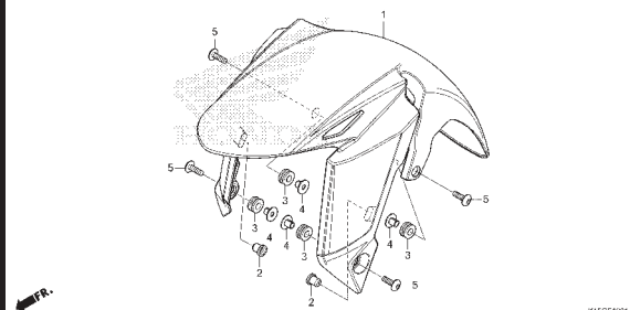
F-10-1 FRONT FENDER(CB150RM)
