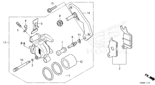
F-17 REAR BRAKE CALIPER
