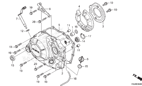
E-10 LEFT CRANKCASE COVER
