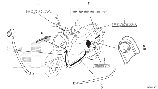
F-48-1 MARK/STRIPE(2)
