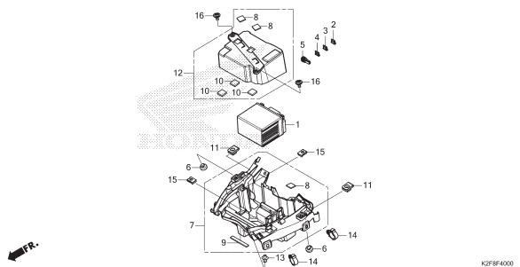
F-40 BATTERY
