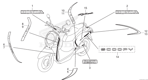
F-48-2 MARK/STRIPE(3)
