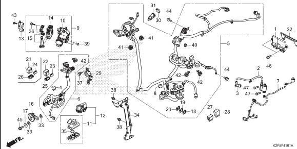
F-41-1 WIRE HARNESS(ACF110CBT-2IN,4IN)
