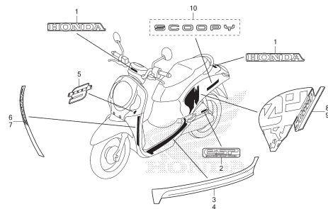
F-48 MARK/STRIPE(1)
