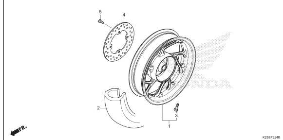
F-22-40 REAR WHEEL(ACB160CAT)
