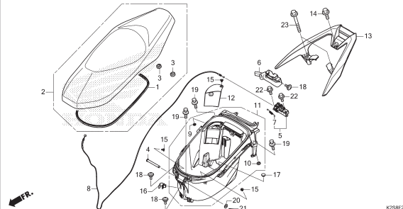
F-24 SEAT/LUGGAGE BOX
