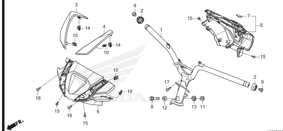
F-9-1 HANDLE PIPE/HANDLE COVER (ACB160CBT)
