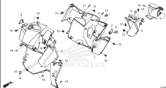
F-13 INNER COVER
