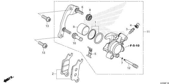
F-18-1 FRONT BRAKE CALIPER (ACB160CBT)
