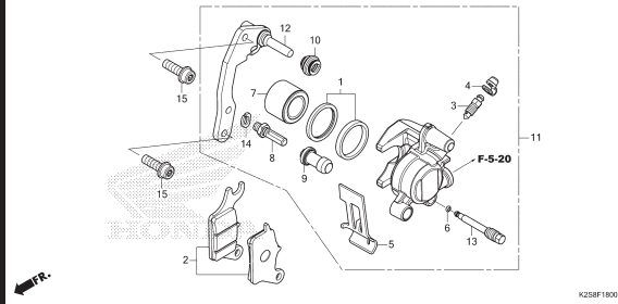
F-18 FRONT BRAKE CALIPER(ACB160CAT)
