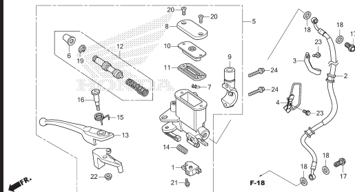
F-5-10 FRONT BRAKE MASTER CYLINDER
