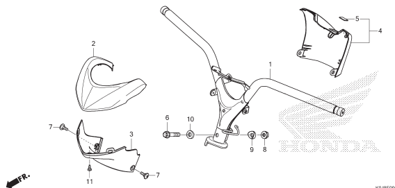
F-12 FRONT COVER/INNER COVER (ACJ110CBFL/CBFM/CBTL/CBTM)
