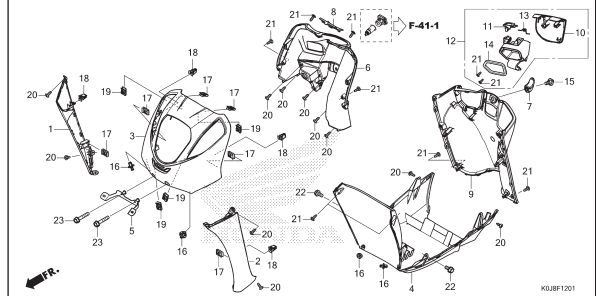
F-12-1 FRONT COVER/INNER COVER (ACJ110CBFN/CBTN)
