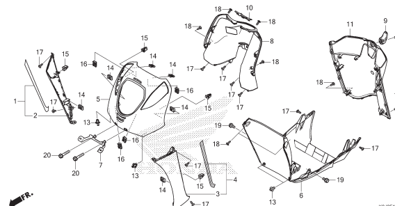
F-12 FRONT COVER/INNER COVER (ACJ110CBFL/CBFM/CBTL/CBTM)
