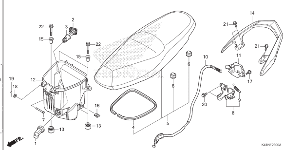
F-23 SEAT/LUGGAGE BOX
