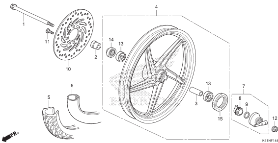
F-14-40 FRONT WHEEL(CAST)
