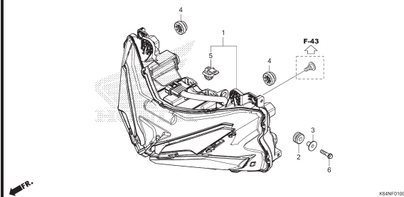
F-1 HEADLIGHT
