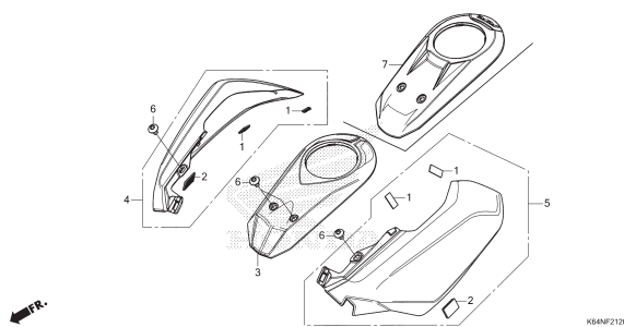
F-21-20 TANK COVER
