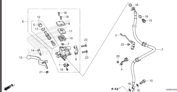
F-5 FRONT BRAKE MASTER CYLINDER (CBR250S3)
