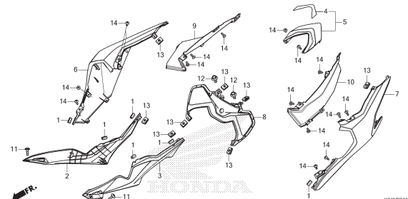
F-24 SIDE COVER/REAR COWL (CBR250S3L/S3M/S3AL/S3AM)
