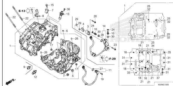
E-15 CRANKCASE
