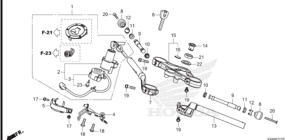
F-7 HANDLE PIPE/TOP BRIDGE
