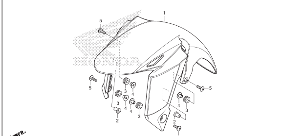
F-10 FRONT FENDER (CBR250S3L/S3M/S3AL/S3AM)
