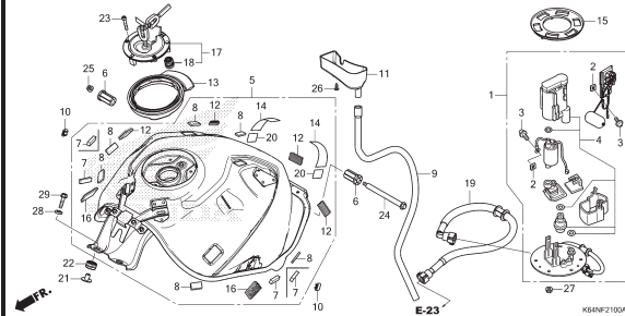
F-21 FUEL TANK/FUEL PUMP
