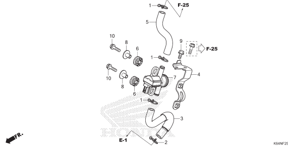
F-25-20 AIR INJECTION SOLENOID VALVE
