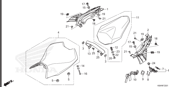
F-23-1 SEAT(CBR250S3P/S3AP)
