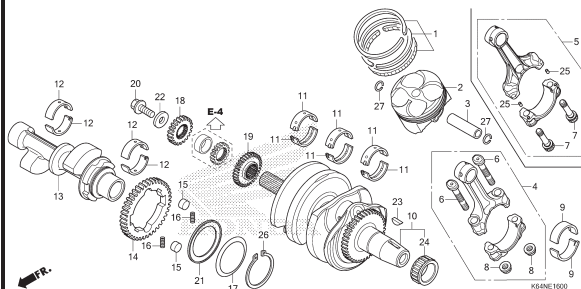
E-16 CRANKSHAFT/PISTON
