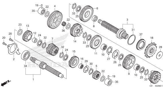
E-17 TRANSMISSION
