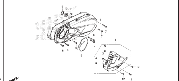
E-13 LEFT SIDE COVER
