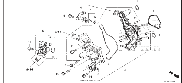
E-9 WATER PUMP
