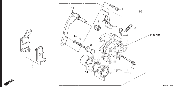
F-18-1 FRONT BRAKE CALIPER (CBS)
