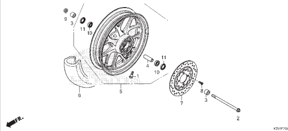
F-22-40 REAR WHEEL (CAST/DISK BRAKE)
