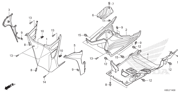
F-14 FLOOR STEP (ACB125CBFL,M,N/CBTL,M,N)
