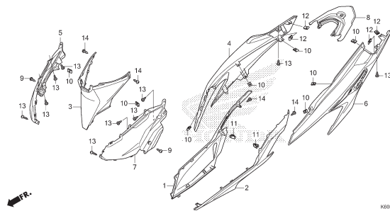
F-15 BODY COVER (ACB125CBFL,M,N/CBTL,M,N)
