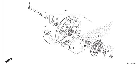
F-20-40 FRONT WHEEL (ACB125CBFL,M,N/CBTL,M,N)
