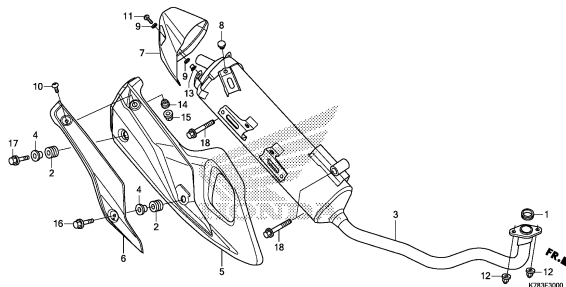
EXHAUST MUFFLER
