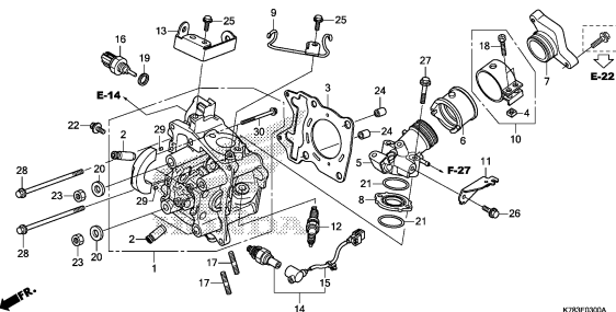
CYLINDER
