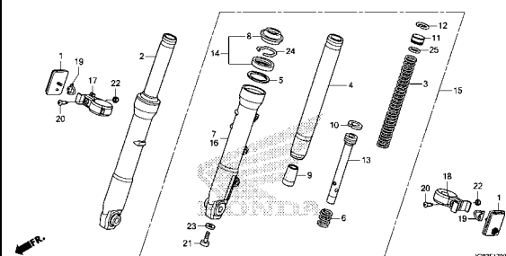
FRONT FORK
