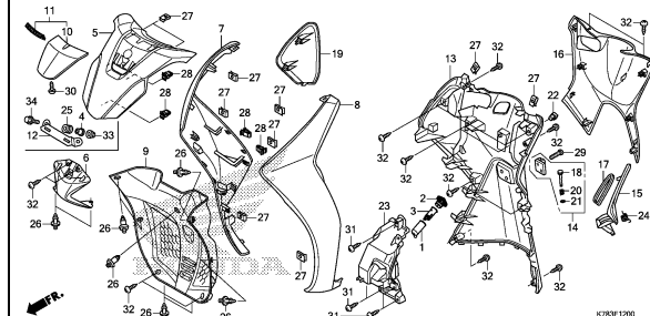
BODY COVER
