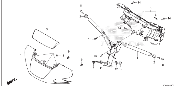
F-9 HANDLE PIPE/HANDLE COVER
