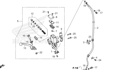
F-5-10 FRONT BRAKE MASTER CYLINDER
