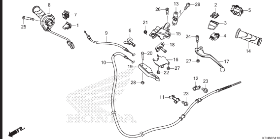
F-4-10 HANDLE LEVER/SWITCH/CABLE
