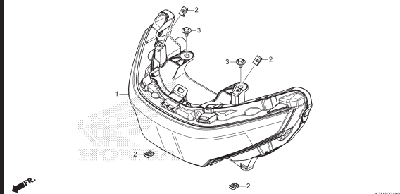
F-1 FRONT COMBINATION LIGHT
