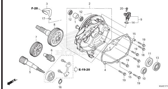
E-17-10 TRANSMISSION
