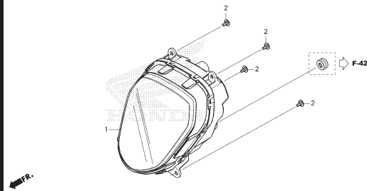
F-1 HEADLIGHT
