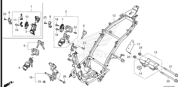
F-42 FRAME BODY
