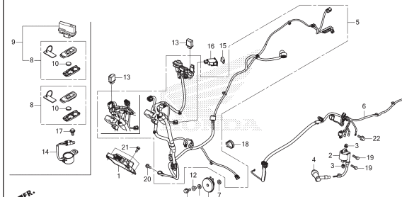
F-41 WIRE HARNESS
