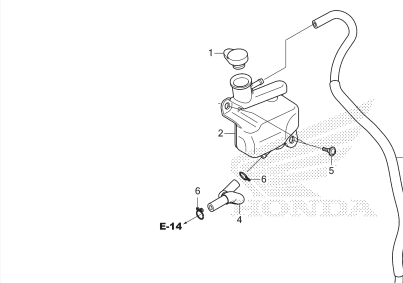
F-43 RESERVE TANK
