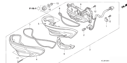
F-28-1 TAILLIGHT (New Tiger Revo)
