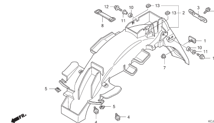
F-26 REAR FENDER
